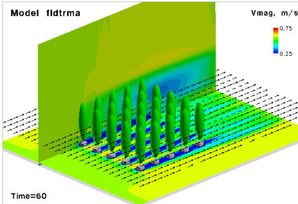
Note: CFD model "fldtrma" used to establish steady-state flow field
